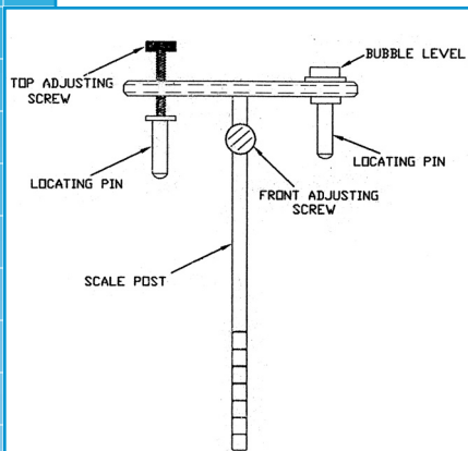
Schematic of Blood Donor Scale Support Post shown above
